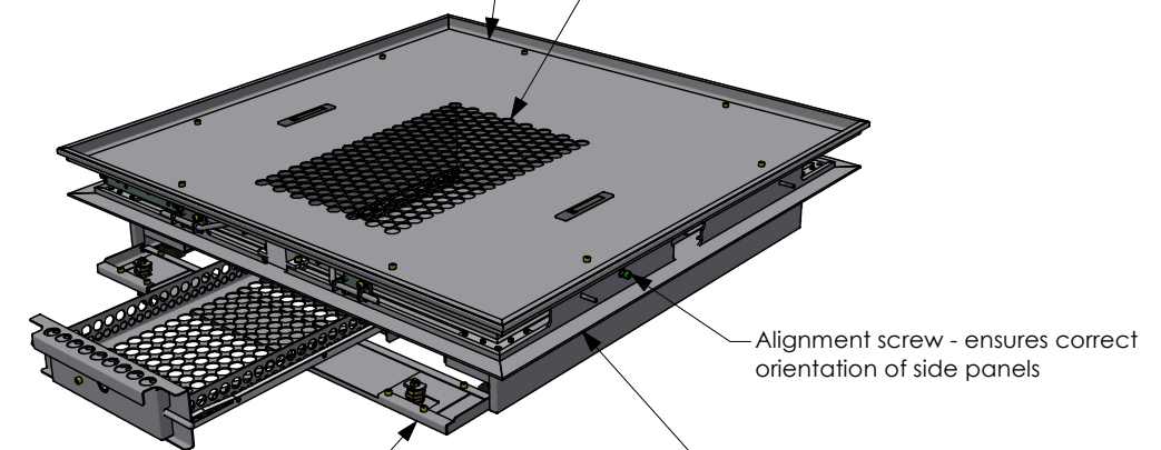
BOTTOM STRUCTURE
