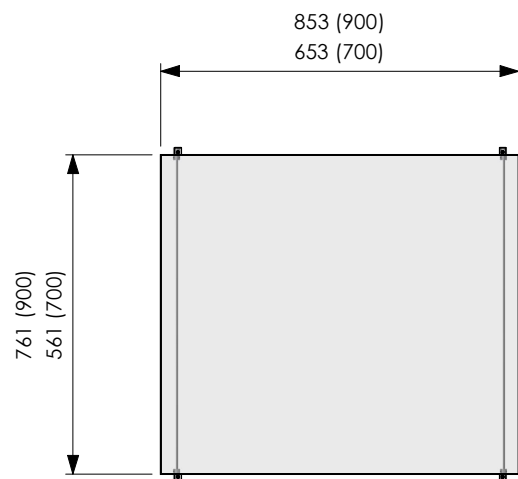
HANGING ROD SHELVING
